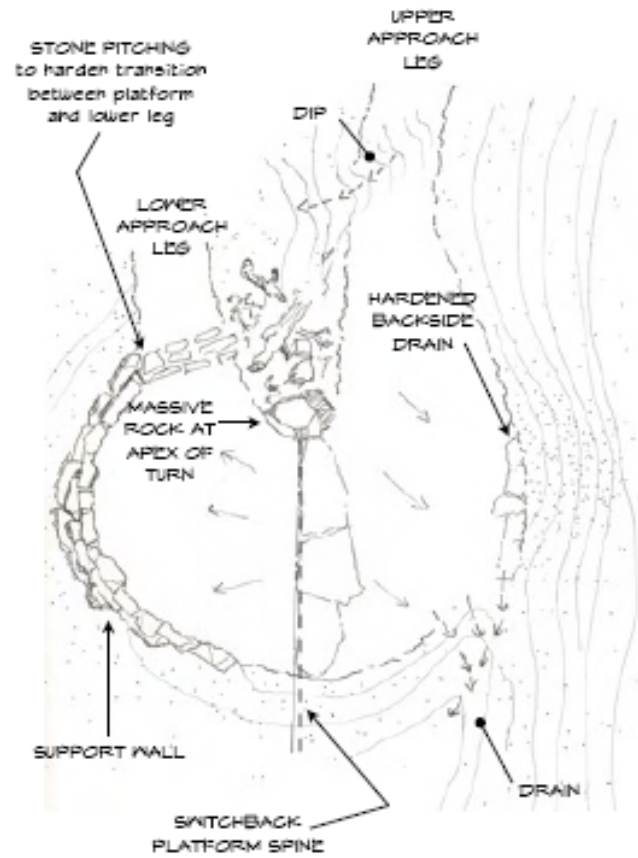
FIGURE 6. Plan View of Switchback
