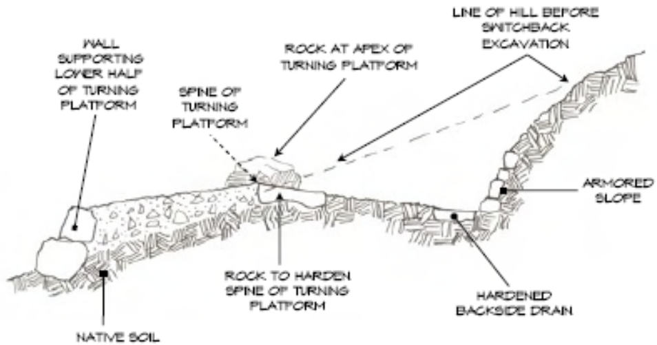
FIGURE 7. Cross-section View of Switchback (slopes away from spine exaggerated)
